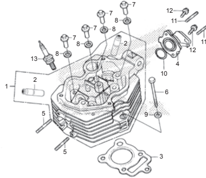
CYLINDER HEAD
