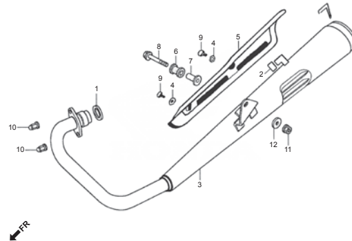
F - 17 MUFFLER ASSY EXHAUST F 05
