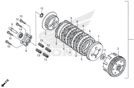
CLUTCH ASSY
