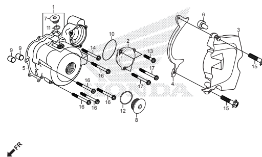
COVER, LEFT CRANKCASE
