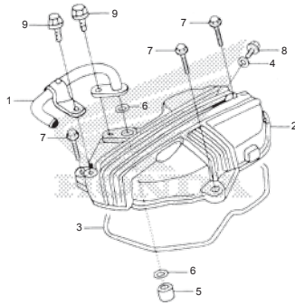
CYLINDER HEAD COVER
