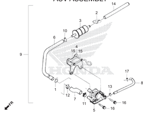
ASV ASSEMBLY
