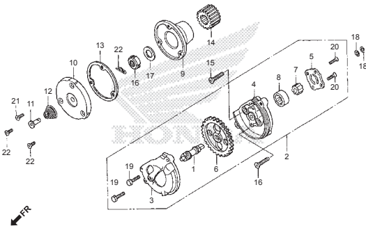
OIL PUMP ASSY
