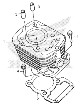
CYLINDER
