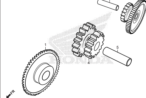
STARTING GEAR
