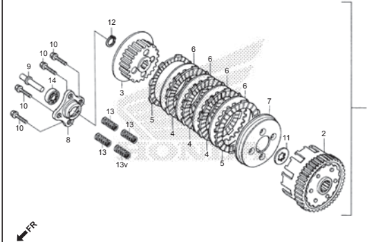
CLUTCH ASSY
