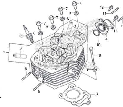
CYLINDER HEAD
