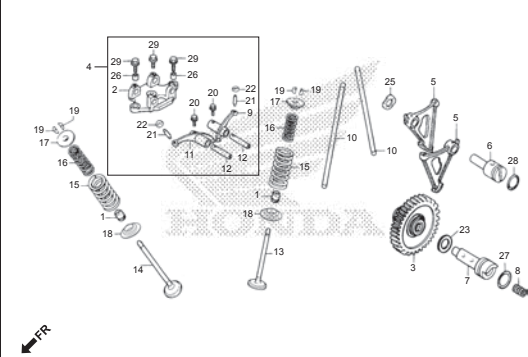
CAMSHAFT-VALVE
