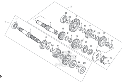
TRANSMISSION
