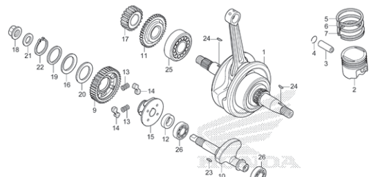
CRANKSHAFT/PISTON/BALANCER
