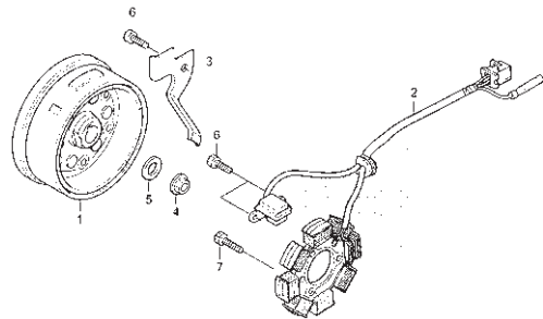
GENERATOR
