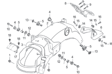
REAR FENDER
