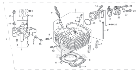
CYLINDER HEAD
