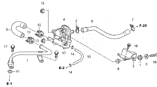
AIR SUCTION VALVE
