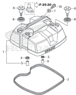
CYLINDER HEAD COVER
