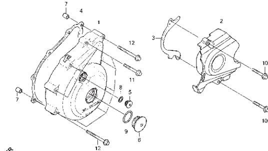
LEFT CRANKCASE COVER
