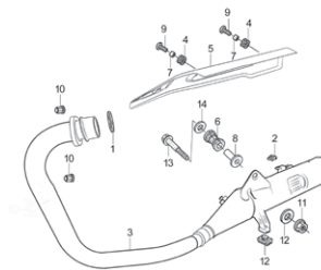
EXHAUST MUFFLER
