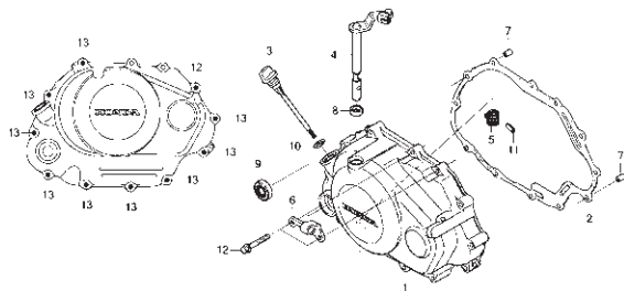
RIGHT CRANKCASE COVER
