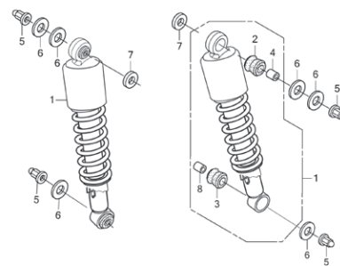
REAR CUSHION
