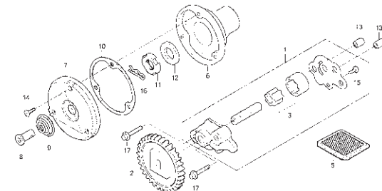
OIL PUMP
