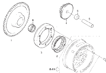
STARTING CLUTCH
