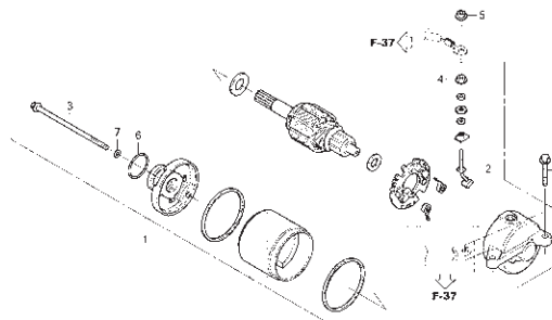
STARTER MOTOR
