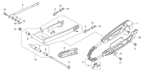
SWINGARM
