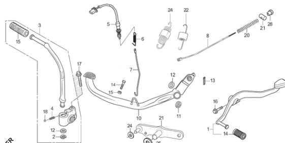
PEDAL
