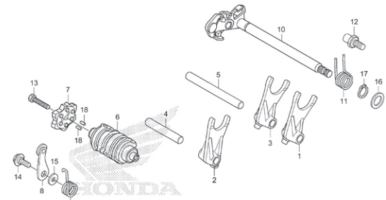
GEARSHIFT DRUM
