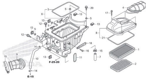
AIR CLEANER
