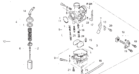
CARBURETOR
