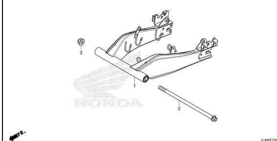
REAR CUSHION
