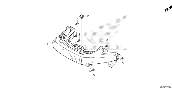
REAR COMBINATION LIGHT
